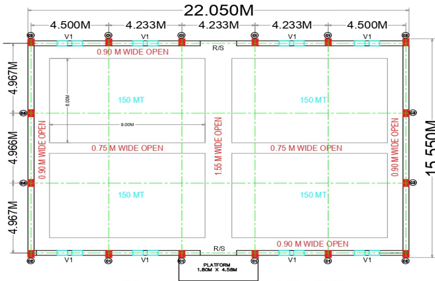
PLAN FOR 1/600 MT.UNIT
